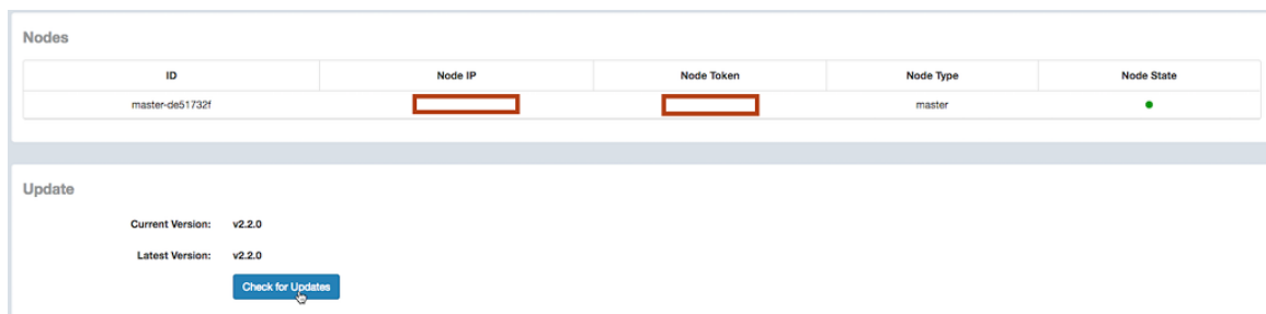
Figure 20: Updating software
