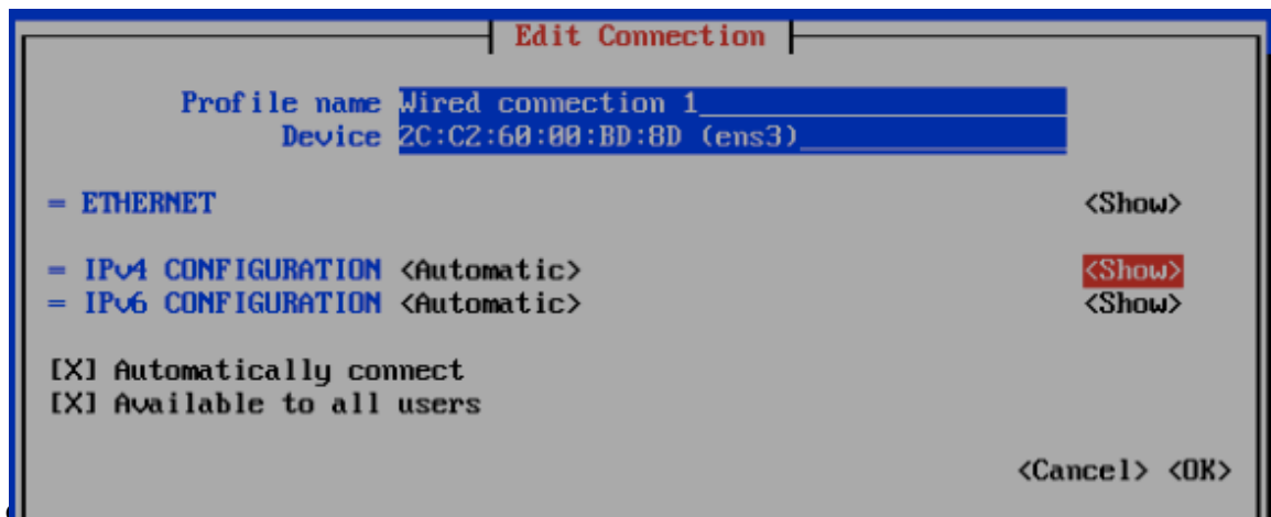
Figure 7: Edit
